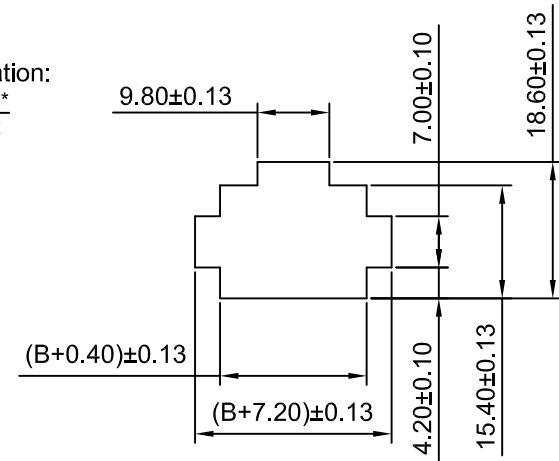
Panel Hole Layout Thickness:0.50~2.00mm
