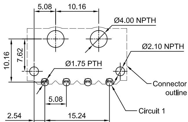
P.C.B LAYOUT(TOP VIEW) TOLERANCE:±0.05
