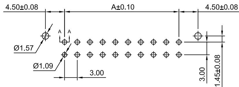
P.C.B LAYOUT TOLERANCE: ±0.05
