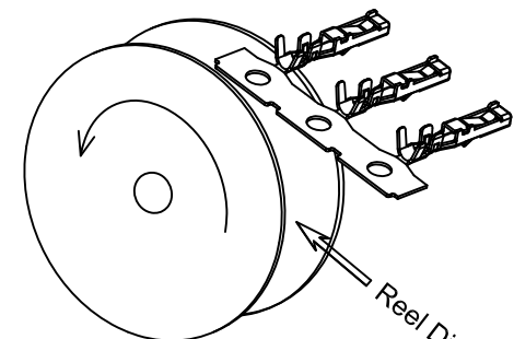
Winding Direction
