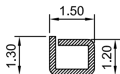
SEC:C-C
