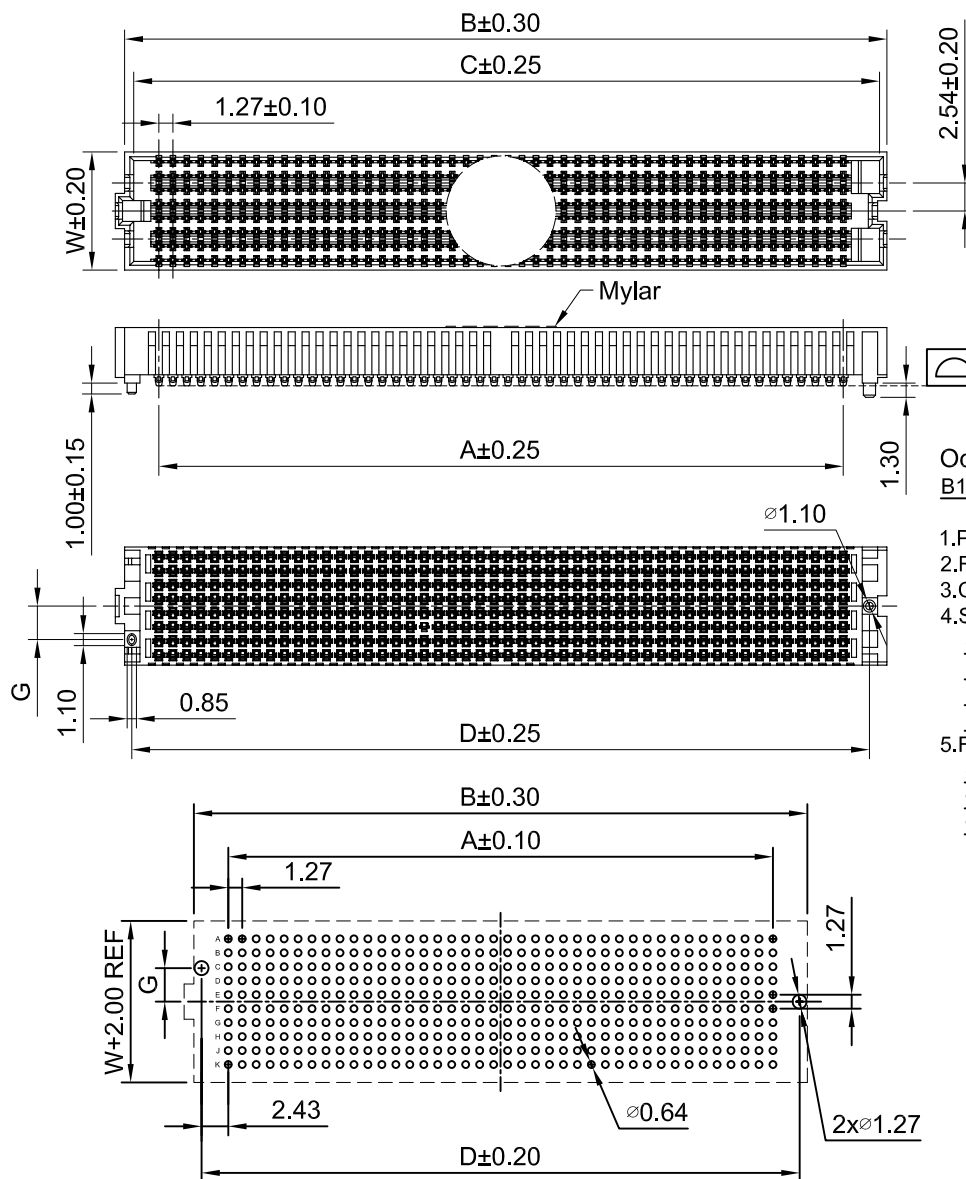
P.C.B LAYOUT(TOP VIEW ) TOLERANCE:±0.05
