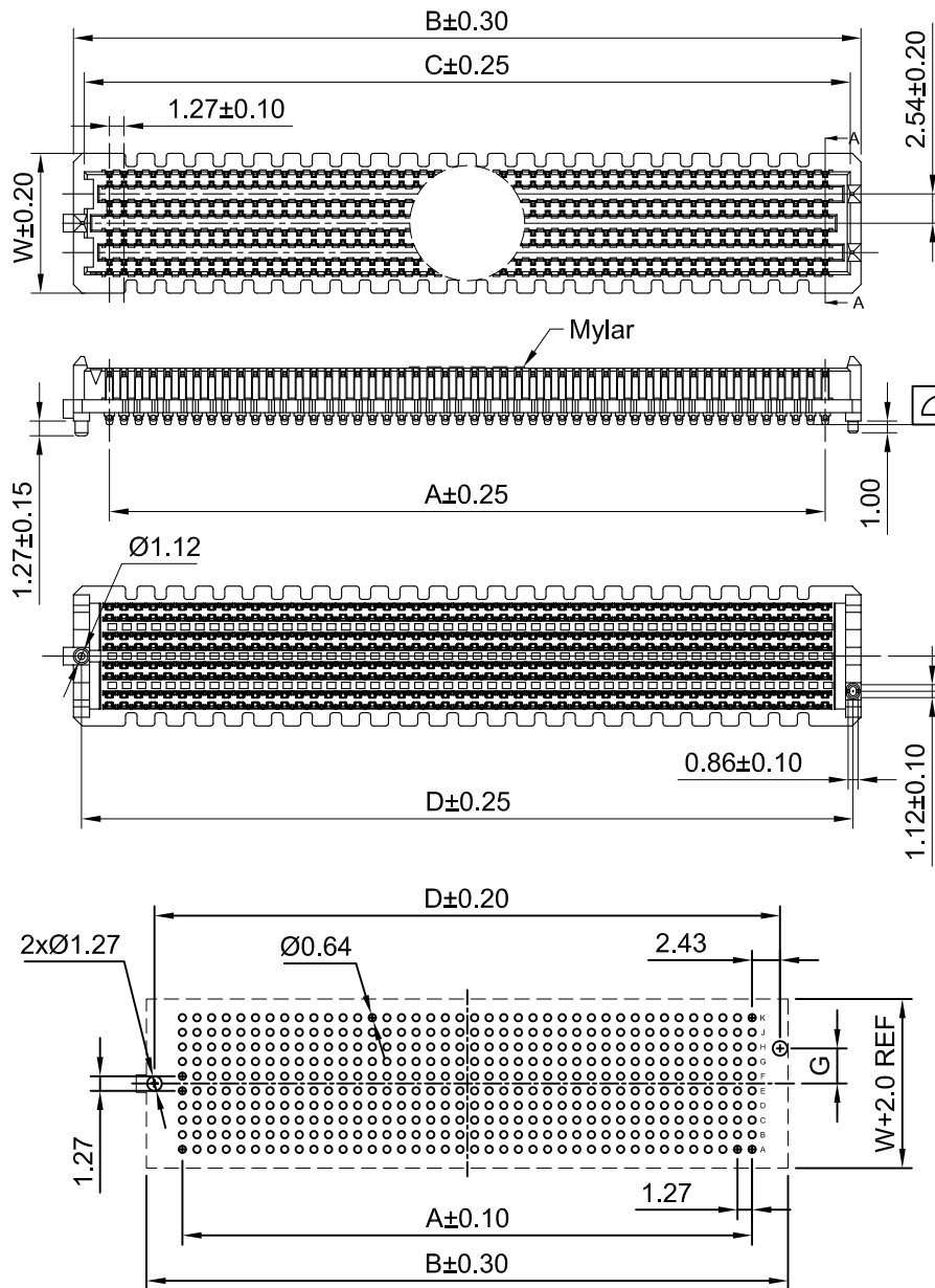
P.C.B LAYOUT (TOP VIEW) TOLERANCE: ±0.05
