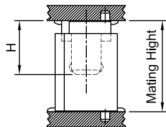
ASSEMBLY LAYOUT MATED WITH B0802WVM-S-2xXP
