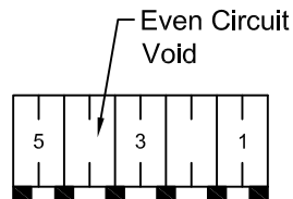
-A Type Just for odd numbers (For example,5P-0A-*-**-A)
