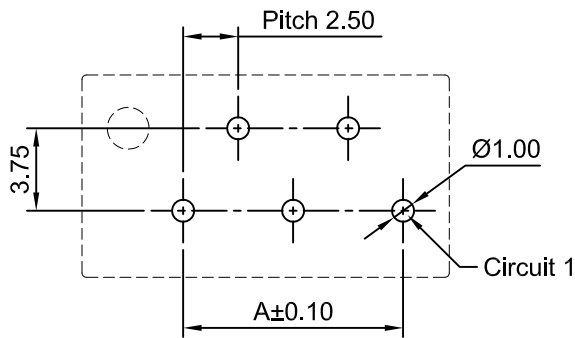
Odd Numbers Component Side [A7921WVI-XP-**]
