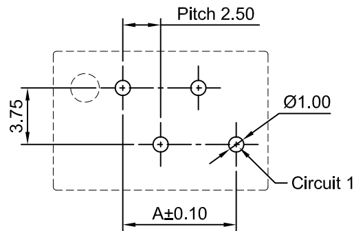
Even Numbers Component Side [A7921WVI-XP-**-2]
