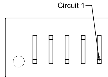
Odd Numbers Solder Side [A7921WVI-XP-**-2]
