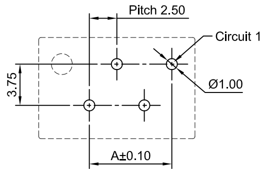
Even Numbers Component Side [A7921WVI-XP-**]
