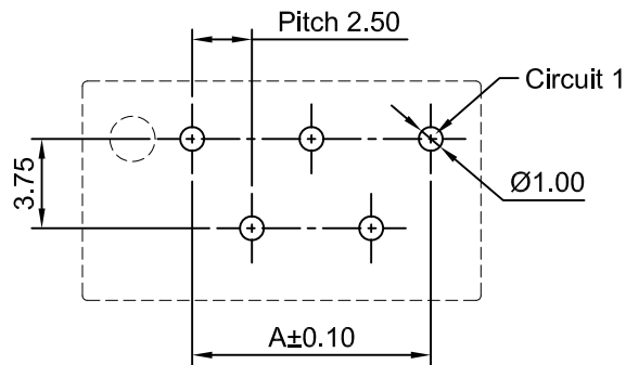
Odd Numbers Component Side [A7921WVI-XP-**-2]
