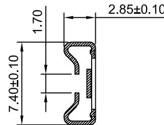
SEC:C-C
