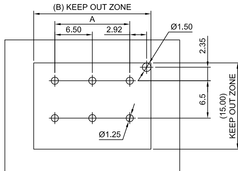
P.C.B LAYOUT TOLERANCE:±0.05
