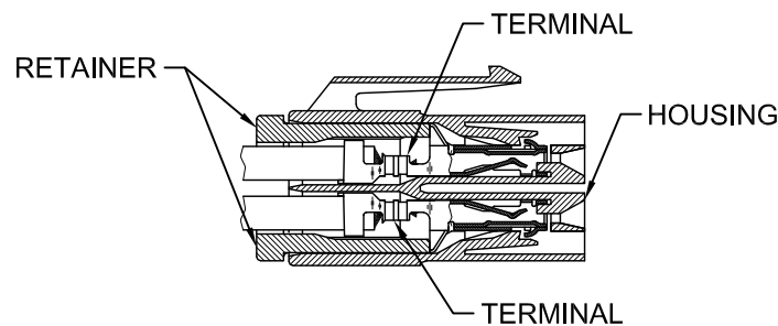
TERMINAL & RETAINER ASSEMBLY DRAWING
