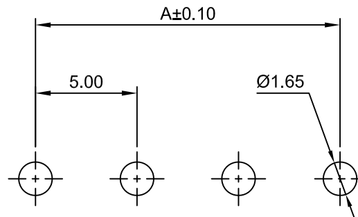
P.C.B LAYOUT TOLERANCE:±0.05
