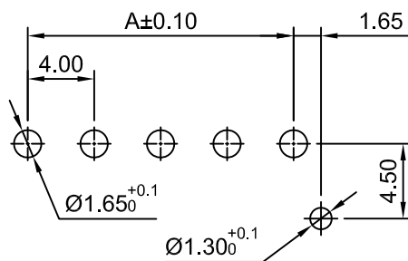
P.C.B LAYOUT TOLERANCE:±0.05
