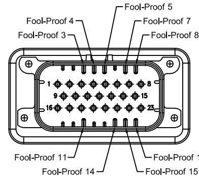
23-POSITION CONNECTOR FOOL-PROOF LOCATIONS
