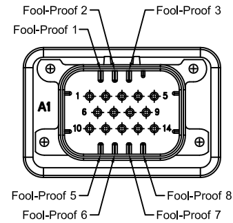
14-POSITION CONNECTOR FOOL-PROOF LOCATIONS
