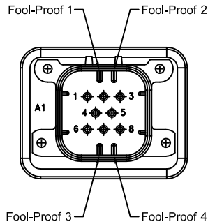
8-POSITION CONNECTOR FOOL-PROOF LOCATIONS
