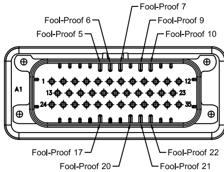
35-POSITION CONNECTOR FOOL-PROOF LOCATIONS
