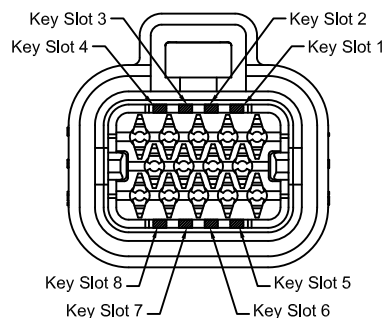
14-POSITION CONNECTOR KEY SLOT LOCATIONS
