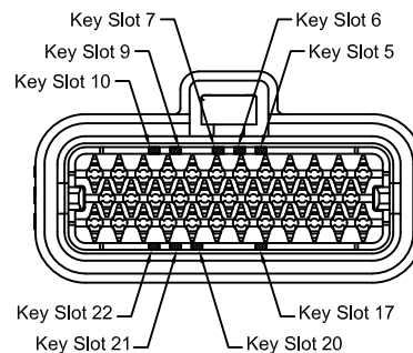
35-POSITION CONNECTOR KEY SLOT LOCATIONS
