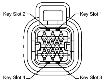
8-POSITION CONNECTOR KEY SLOT LOCATIONS
