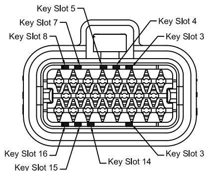
23-POSITION CONNECTOR KEY SLOT LOCATIONS
