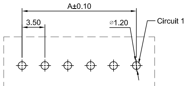
P.C.B LAYOUT TOLERANCE:±0.05
