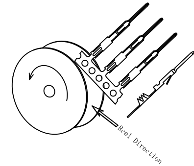
Winding Direction
