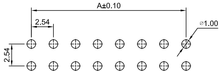
P.C.B LAYOUT TOLERANCE:±0.05
