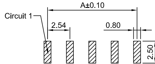
P.C.B LAYOUT (TOP VIEW) TOLERANCE:±0.05
