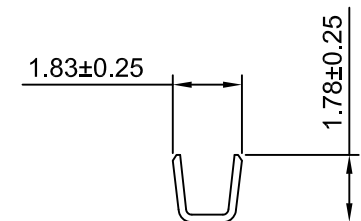
SEC:C-C
