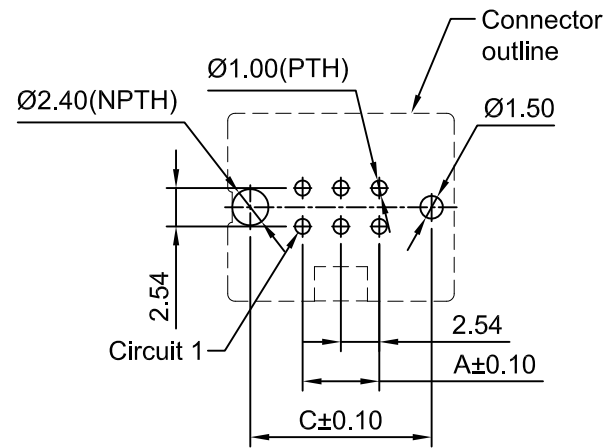
P.C.B LAOUT (TOP VIEW) TOLERANCE:±0.05
