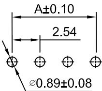
P.C.B LAYOUT TOLERANCE:±0.05
