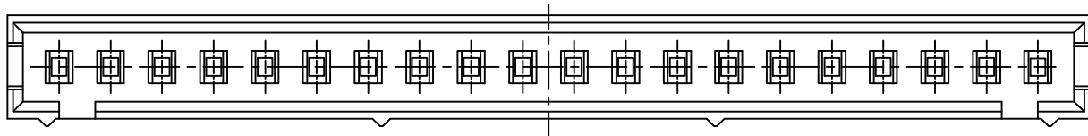
20P-36P(Four ribs)
