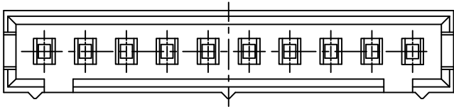
10P-19P(Three ribs)
