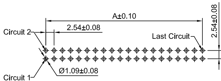
P.C.B LAYOUT TOLERANCE:±0.05
