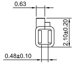
SEC:C-C
