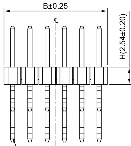
Pin 0.64 SQ
