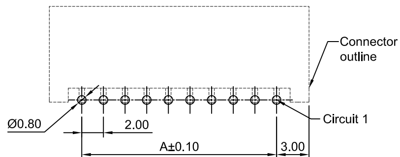
P.C.B LAYOUT (TOP VIEW) TOLERANCE:±0.05
