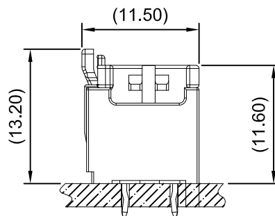
Mated Drawing (REF)
