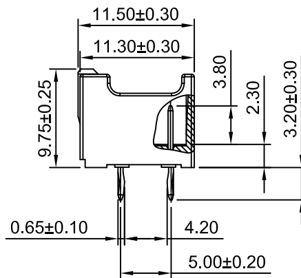
Mated Drawing (REF)
