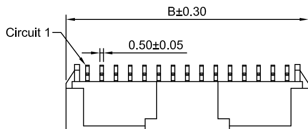
P.C.B LAYOUT TOLERANCE:±0.05
