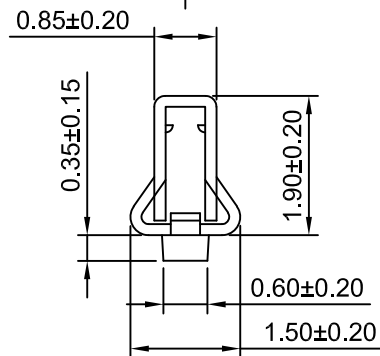
SEC: C-C
