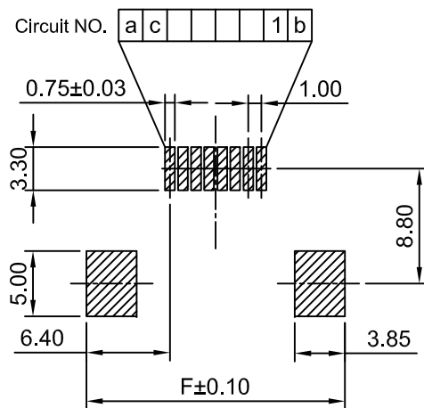
P.C.B LAYOUT TOLERANCE:±0.05
