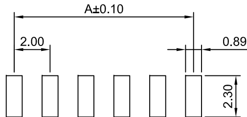
P.C.B LAYOUT TOLERANCE:±0.05
