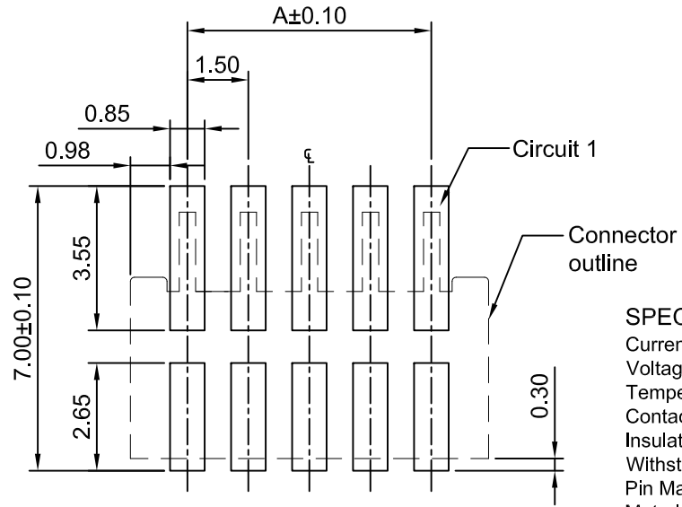
P.C.B LAYOUT (TOP VIEW) TOLERANCE: ±0.05
