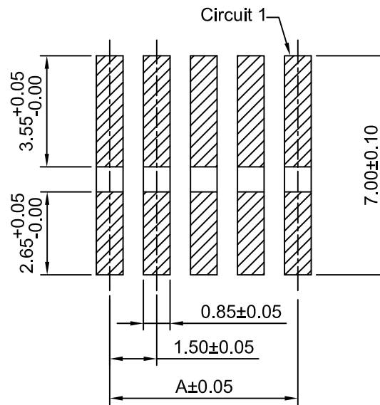
PCB LAYOUT
