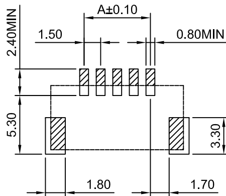
P.C.B LAYOUT TOLERANCE:±0.05
