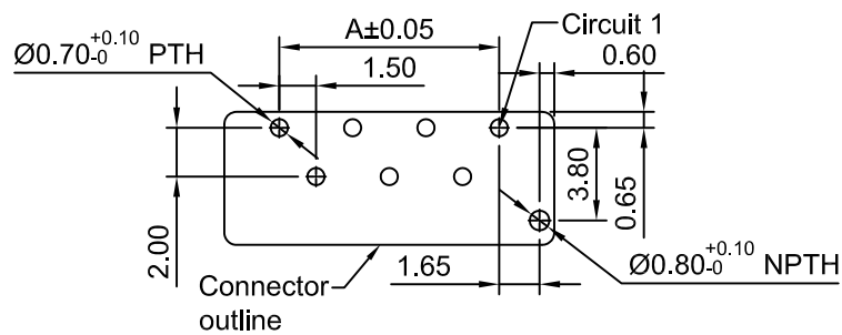
P.C.B LAYOUT(TOP VIEW) TOLERANCE:±0.05
