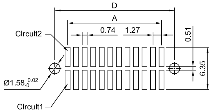
P.C.B LAYOUT(TOP VIEW ) TOLERANCE:±0.05
