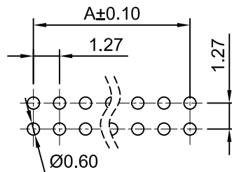
PCB LAYOUT TOLERANCE:±0.05
