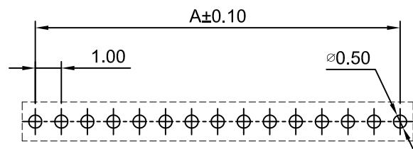
P.C.B LAYOUT TOLERANCE:±0.05
