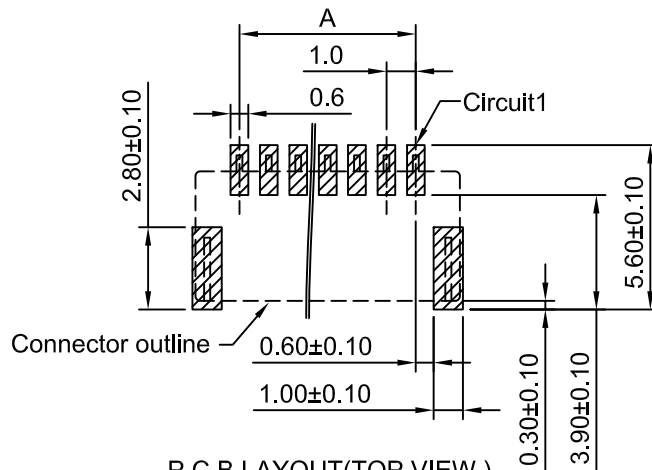
P.C.B LAYOUT(TOP VIEW ) TOLERANCE:±0.05
