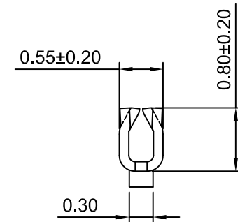
SEC: C-C
