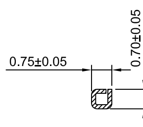
SEC:C-C
