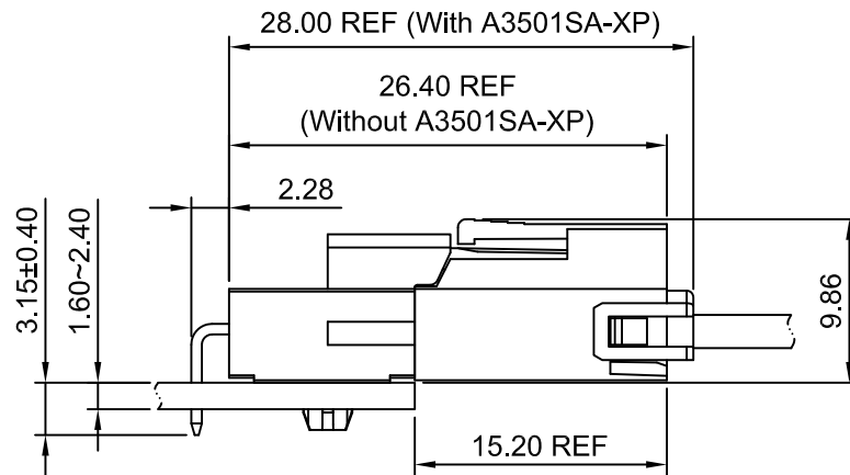
HOUSING BODY FLUSH WITH PCB EDGE
