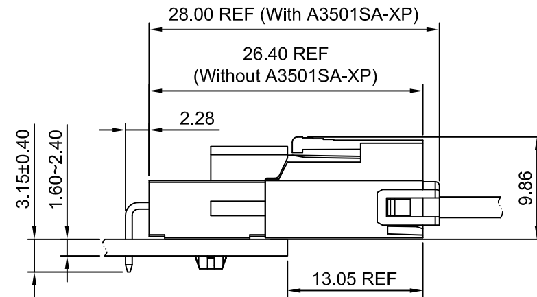
LATCH FLUSH WITH PCB EDGE
