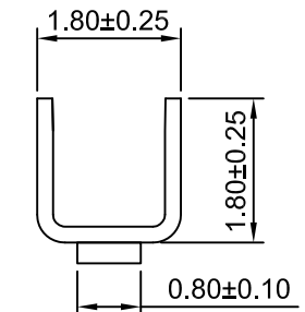
SEC:C-C
